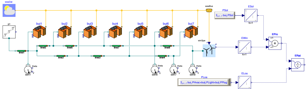
Figure 1: Neighborhood model with renewable energy sources. The yellow lines are weather data, green lines are electrical lines, and dashed blue lines are for post-processing.
