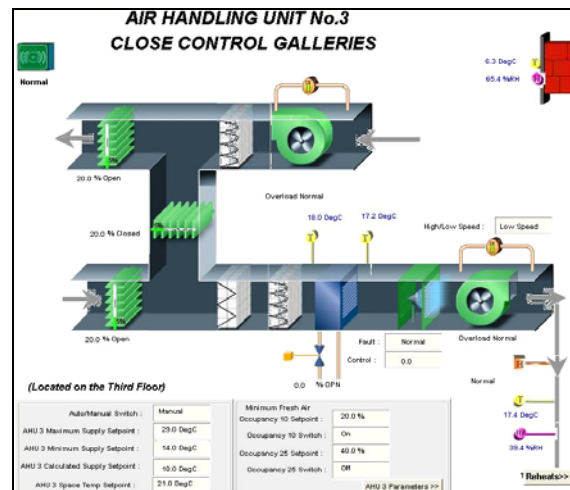
Figure 6 Glucksman Art Gallery's BMS Graphical User Interface
