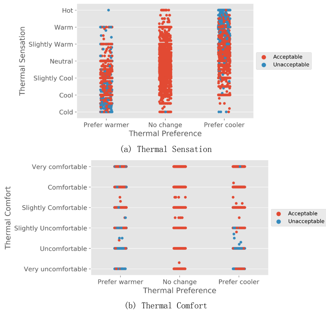
Figure 1. Jitter plots of thermal preference and thermal acceptability votes on (a) thermal sensation scale and (b) thermal comfort scale. Each dot marks an individual vote and the colors indicate the thermal acceptability as described in the legend. Most studies in the ASHRAE Database used thermal comfort scale allowing integer votes only.
