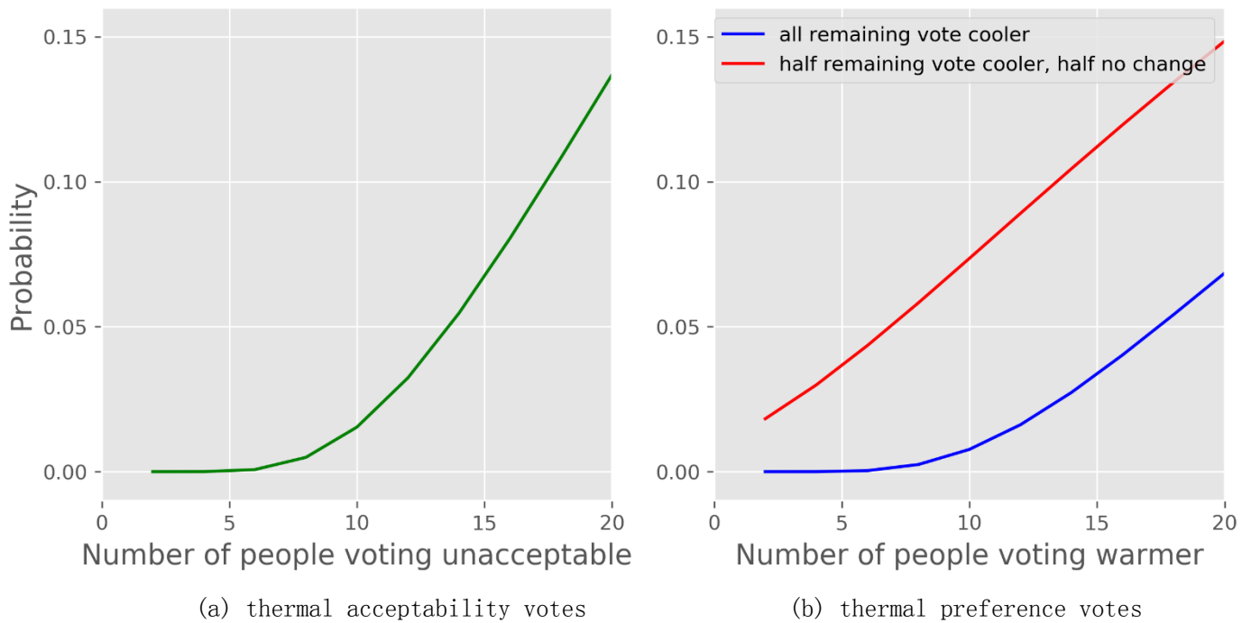
Figure 3. The calculated probability (p-value) of occupants voting unacceptable (left) or for prefer warmer (right) in different hypothetical scenarios (assuming a sample size of 100). The calculated probability increases as the total number of occupants (or neighbors) vote in a similar fashion.
