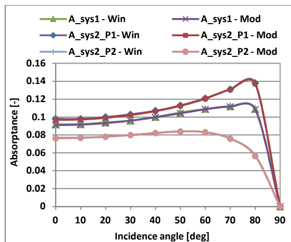
Figure 4 Absorptance values of single (sys1) and double pane (sys2) glazing systems calculated at different incidence angles using WINDOW 6 with spectrally averaged data and Modelica
