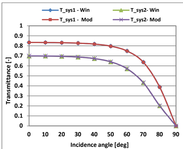
Figure 2 Transmittance values of single (sys1) and double pane (sys2) glazing systems calculated at different incidence angles using WINDOW 6 with spectrally averaged data and Modelica
