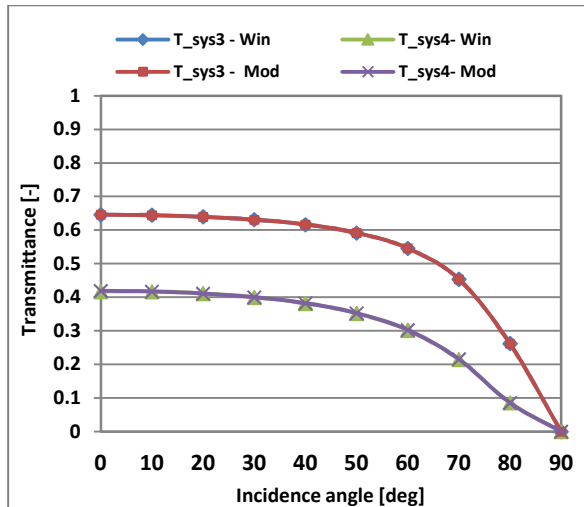
Figure 5 Transmittance values of single (sys3) and double pane (sys4) glazing systems calculated at different incidence angles using WINDOW 6 with spectrally averaged data and Modelica
