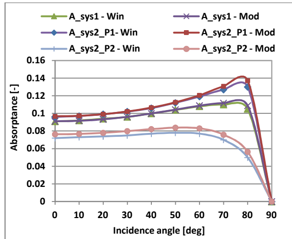
Figure 3 Absorptance values of single (sys1) and double pane (sys2) glazing systems calculated at different incidence angles using WINDOW 6 with spectral data and Modelica
