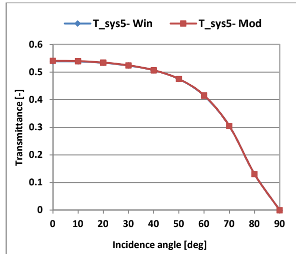
Figure 7 Transmittance values of double pane (sys5) glazing systems calculated at different incidence angles using WINDOW 6 with spectrally averaged data and Modelica
