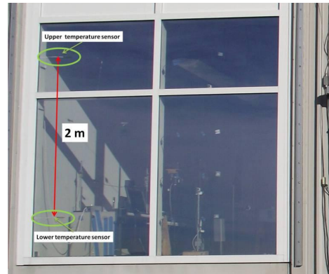
Figure 16 Position of temperature sensors used to measure the outside surface temperature
