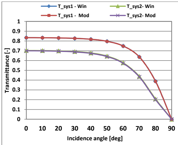
Figure 1 Transmittance values of single (sys1) and double pane (sys2) glazing systems calculated at different incidence angles using WINDOW 6 with spectral data and Modelica
