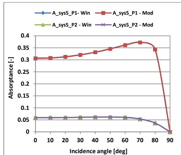
Figure 8 Absorptance values of double pane (sys5) glazing systems calculated at different incidence angles using WINDOW 6 with spectrally averaged data and Modelica
