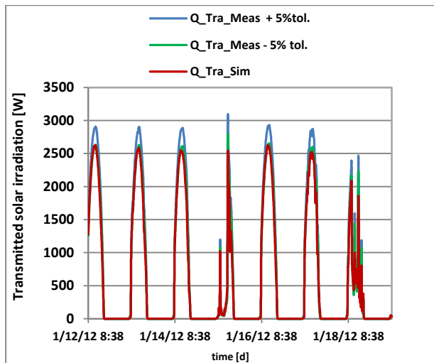
Figure 15 Comparisons between simulated and measured transmitted solar irradiation, considering a 5% tolerance in the LI-COR pyranometers
