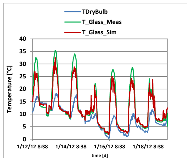
Figure 17 Comparisons between simulated and measured exterior pane outside surface temperature
