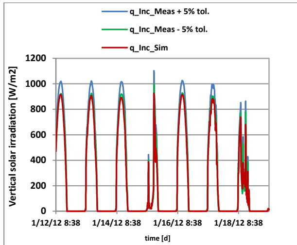
Figure 14 Comparisons between simulated (red) and measured incident vertical outside global irradiation, considering a 5% tolerance in the LI-COR pyranometers
