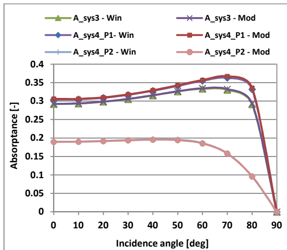
Figure 6 Absorptance values of single (sys3) and double pane (sys4) glazing systems calculated at different incidence angles using WINDOW 6 with spectrally averaged data and Modelica
