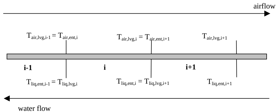
Figure 1: Discrete sections in the cooling coil model
