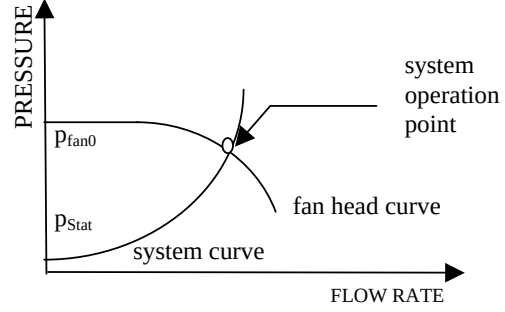
Figure 3 Schematic of the fan model
