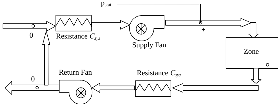
Figure 2: System diagram of the fan-air system simulated in the model
