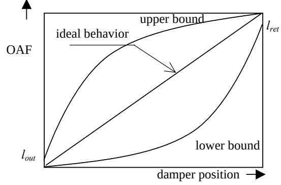
Figure 5: Mixing box performance
