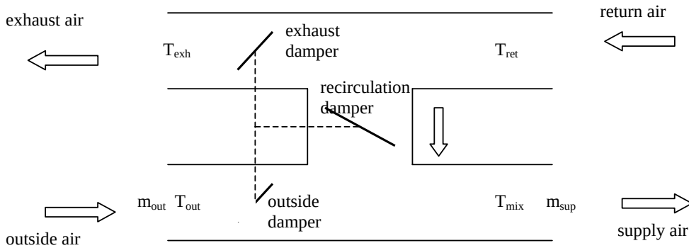
Figure 4: Flow directions and temperatures in a mixing box
