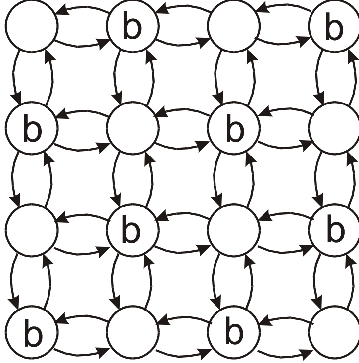
Figure 5. Graph for Laplace's equation example.
