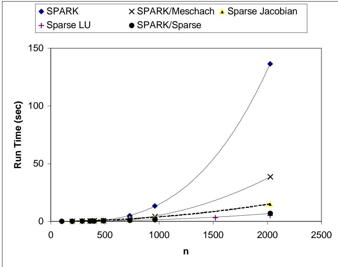
ure 3: Solution times for the Laplace's equation example.
