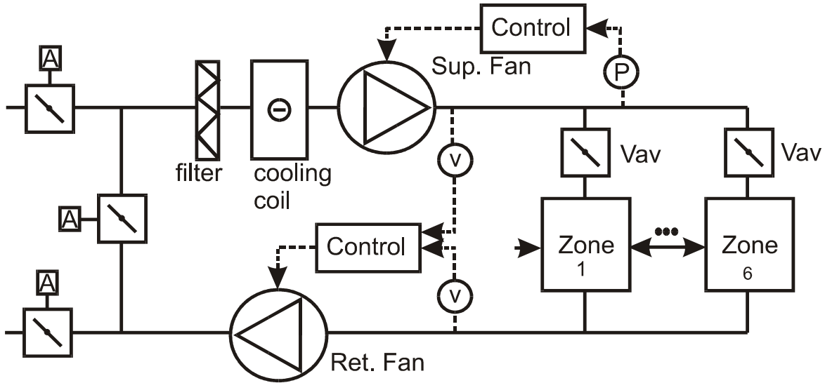
Figure 4 HVAC system.
