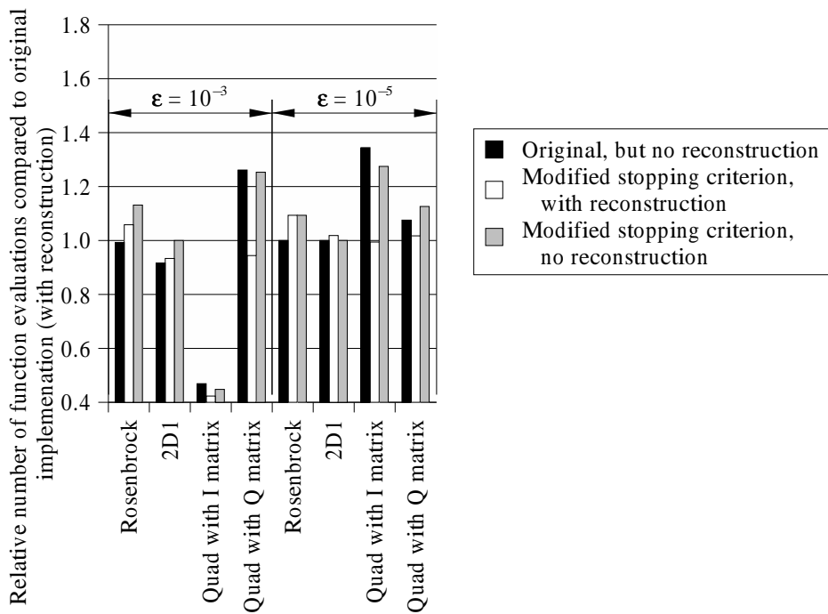
Figure 5.8: Comparison of the benchmark tests.
