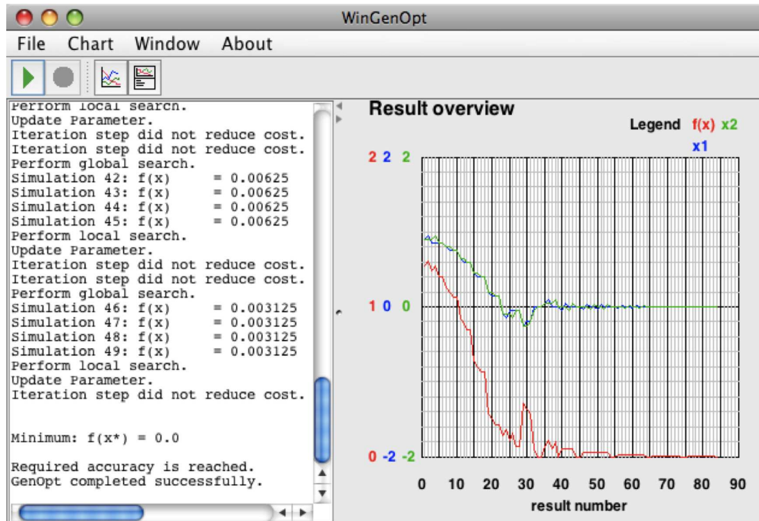
Figure 10.1: Output of GenOpt on Mac OS X for the example file in the directory example/quad/GPSHookeJeeves .
