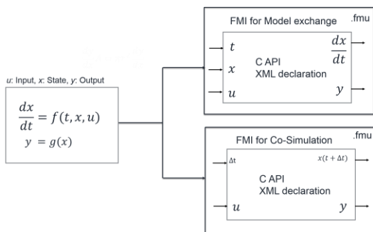
Figure 1 First-order ordinary differential equation exported as an FMU for model exchange (top right) and co-simulation (bottom right).
