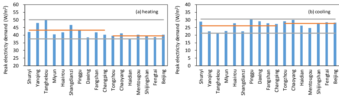
Fig. 12. Simulated peak electricity demand of the reference office building in the year 2000 for different regions of Beijing
