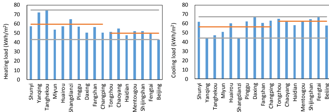
Fig. 10. Simulated loads of the reference office building in the year 2000 for different regions of Beijing
