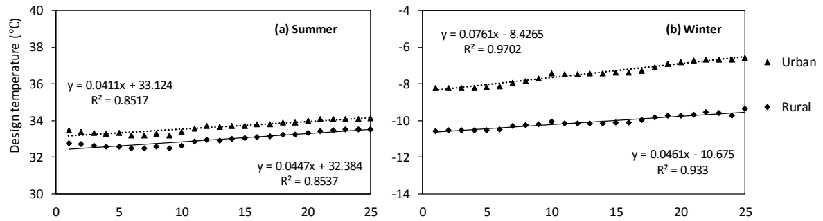
Fig. 9. Design temperature in (a) summer and (b) winter for the urban and rural stations in Beijing
