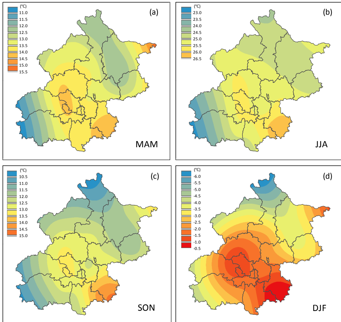
Fig. 2. Spatial distribution of average temperature in (a) March, April, and May (MAM); (b) June, July, and August (JJA); (c) September, October, and November (SON); and (d) December, January, and February (DJF) from 1985 to 2014
