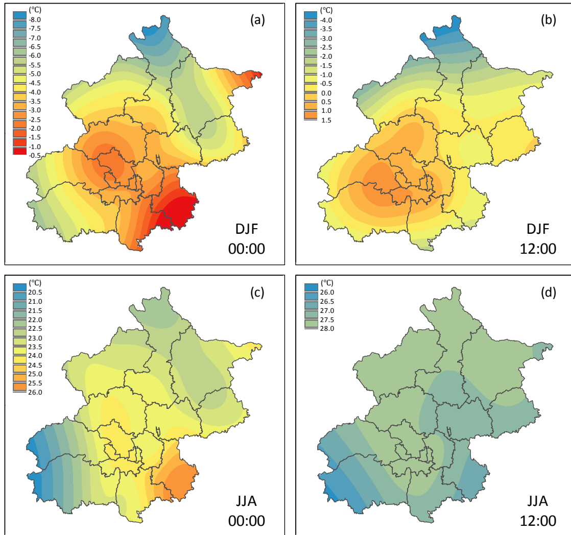
Fig. 3. Spatial distribution of average temperature in (a) DJF 00:00, (b) DJF 12:00, (c) JJA 00:00, and (d) JJA 12:00 from 1985 to 2014
