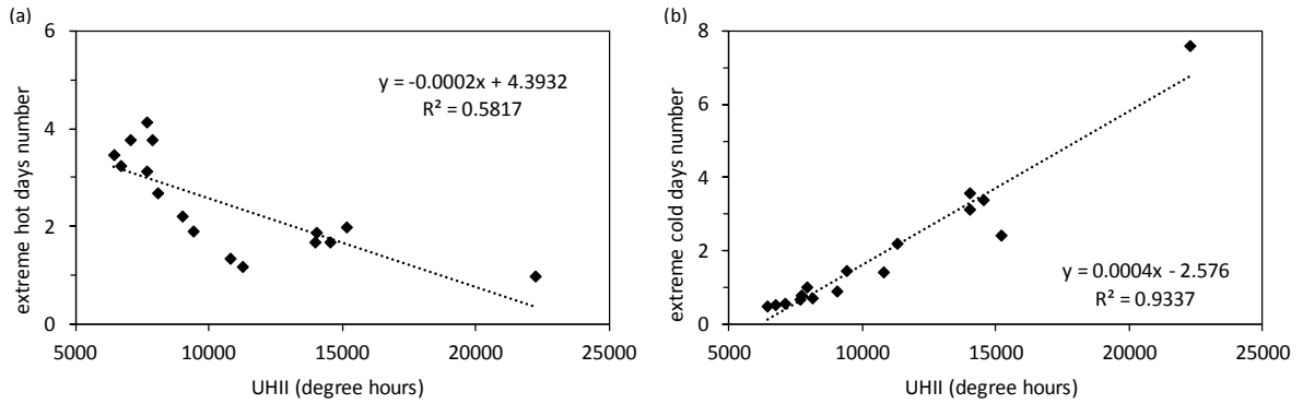
Fig. 8. Relationship between the annual average UHII and (a) the number of extreme hot days or (b) the number of extreme cold days for the 17 stations in Beijing (Each dot on the figure denotes a meteorological station.)
