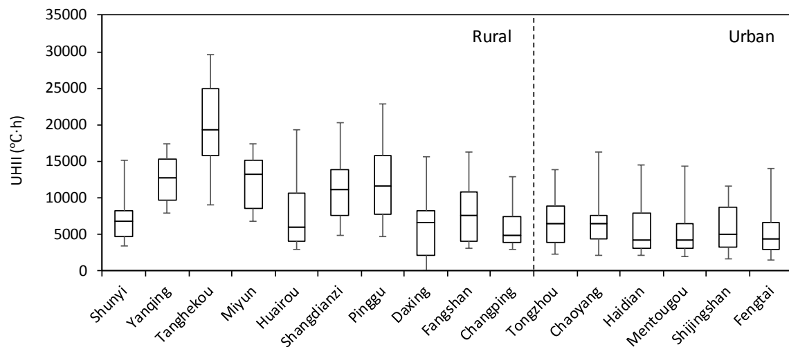
Fig. 5. Boxplot of annual UHII for different weather stations in Beijing from 1985 to 2014
