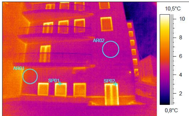
Figure 11 - Thermographic view of northern facade
