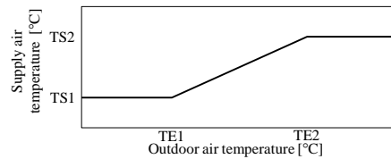
Figure 4- AHU supply air temperature setpoint
