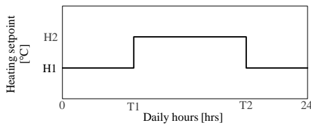
Figure 5 - Daily 24-hour heating setpoint
