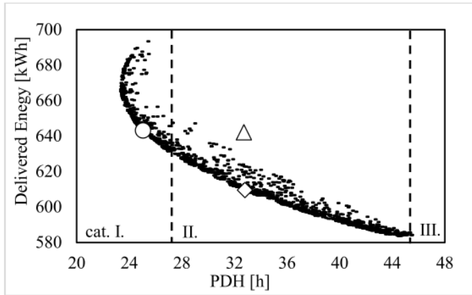
Figure 17- Results of optimization of delivered energy for Zone SW (January)
