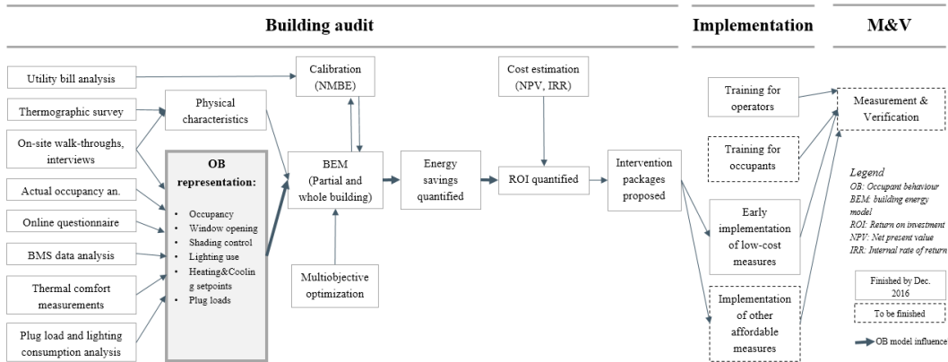
Figure 2. Workflow chart
