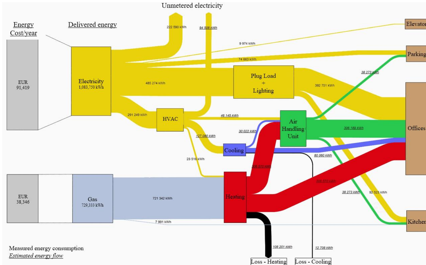
Figure 14 - Sankey diagram of energy use patterns
