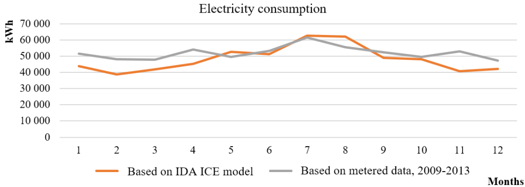
Figure 16 - BEM calibration results for electricity consumption
