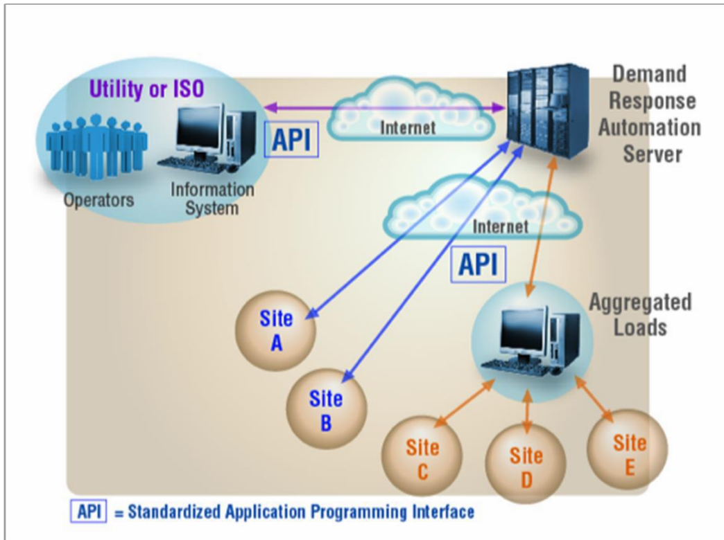
Figure 2. OpenADR is a client server signals system where utility or grid operator's servers send signals to clients who are aggregators, campuses, buildings, or end-use system controls.
