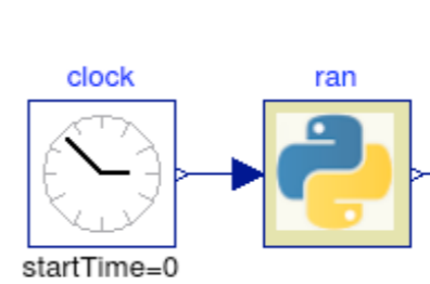
Embedded Python
