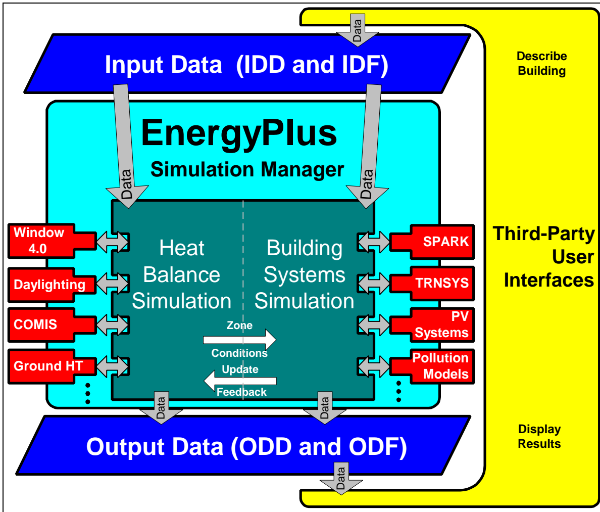
Figure 1 Overall EnergyPlus Structure
