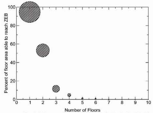
Figure 3 Percentage of floor area that can reach ZEB as a function of number of floors in building: LZEB 2025 Scenario
