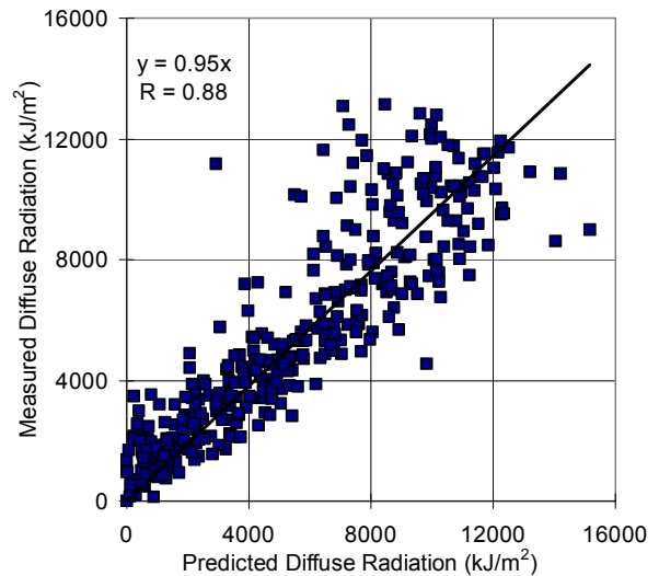
Figure 4. Comparison of predicted to measured daily diffuse solar radiation for Chongqing 1988
