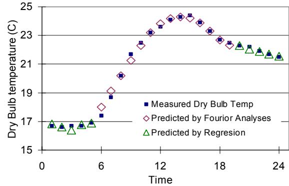
Figure 7. Example of dry-bulb temperature interpolation for Tokyo, December 21
