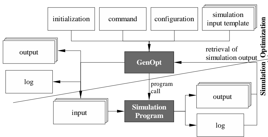
Figure 1: Interface between GenOpt and the simulation program
