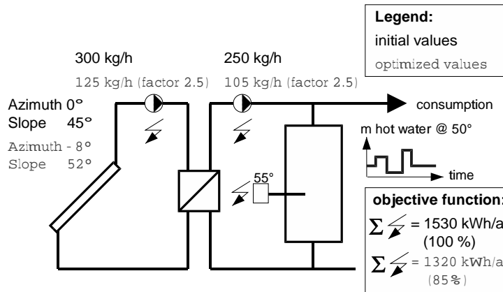
Figure 6: Schematic of the domestic hot water solar system
