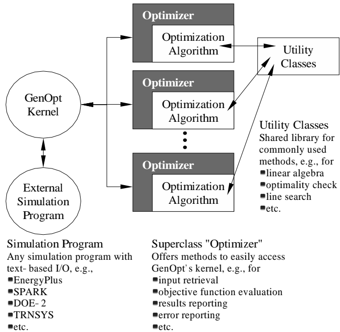
Figure 2: Implementation of minimization algorithms in GenOpt
